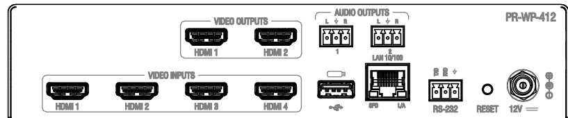
BACK VIEW
