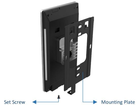
FIG. 2 Mounting Plate
