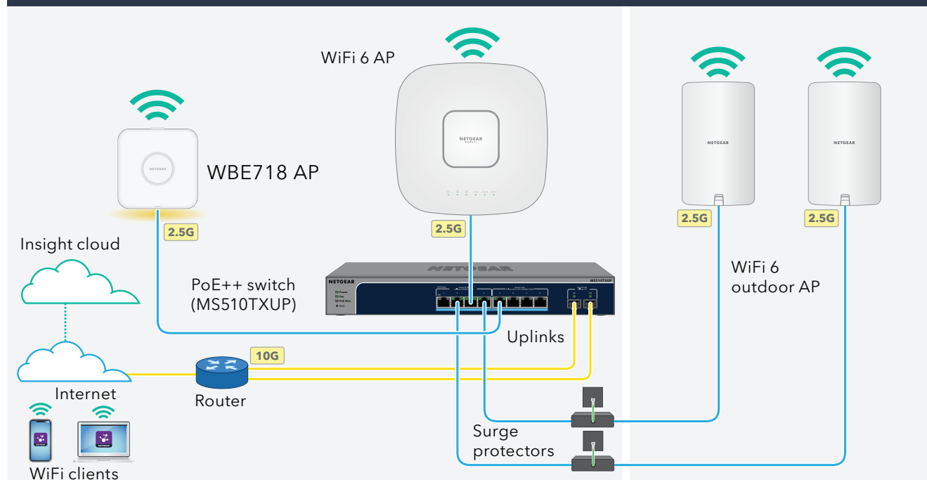
WBE718 Deployment Scenario
