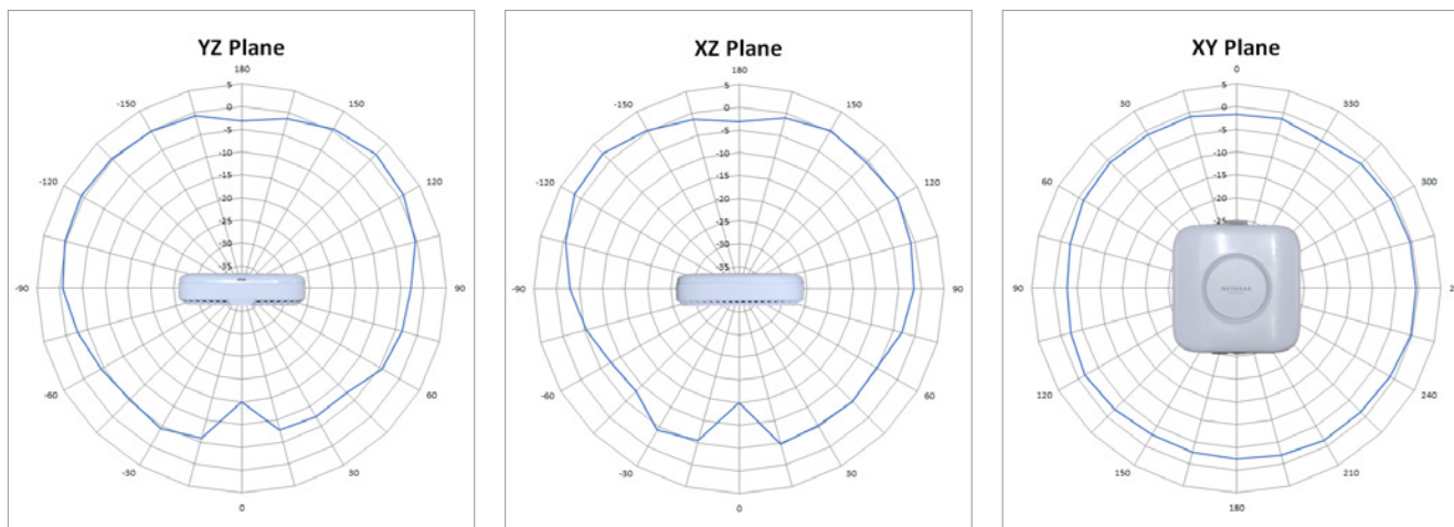
Radio Pattern for 2.4GHz
